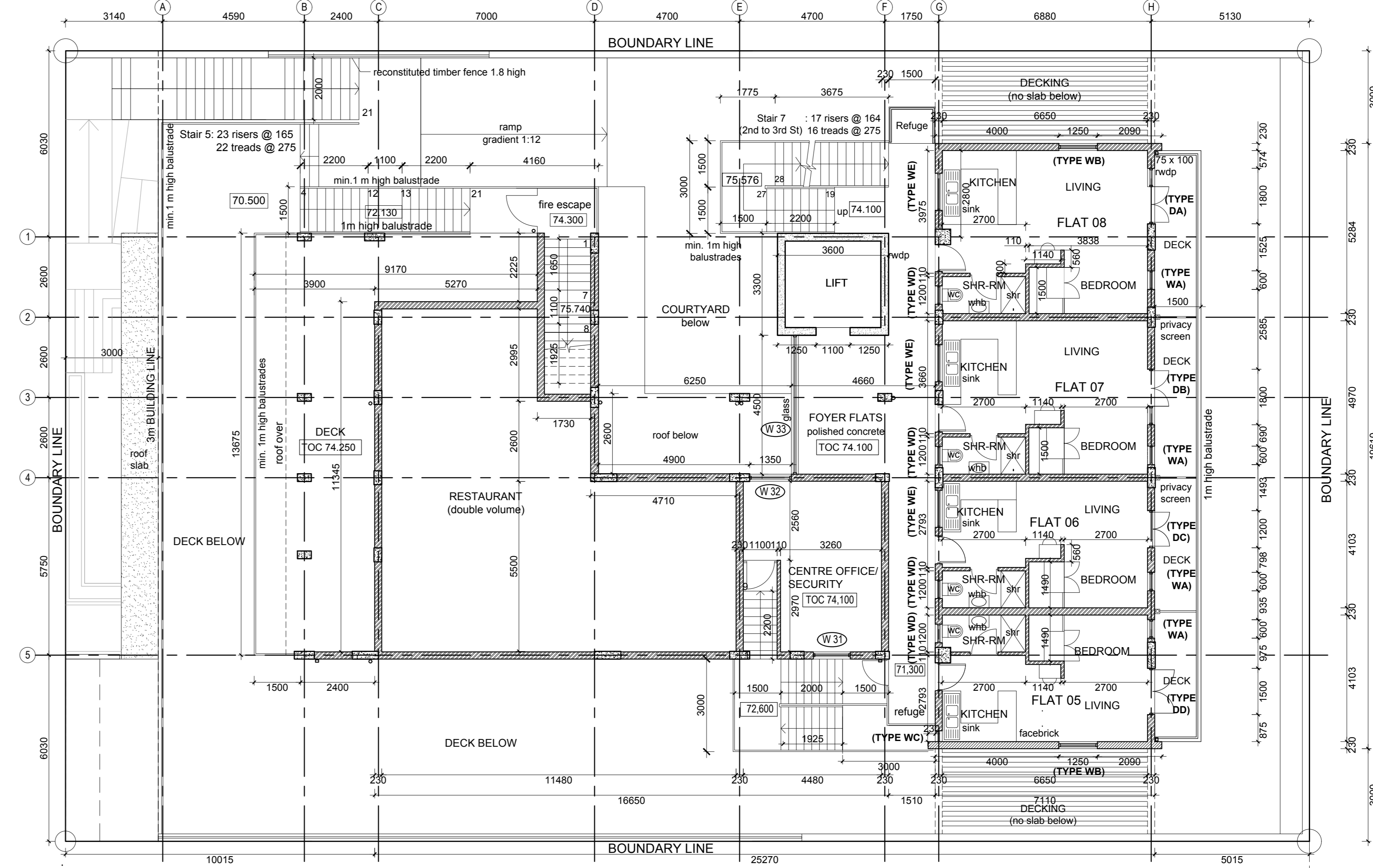
SECOND STOREY
