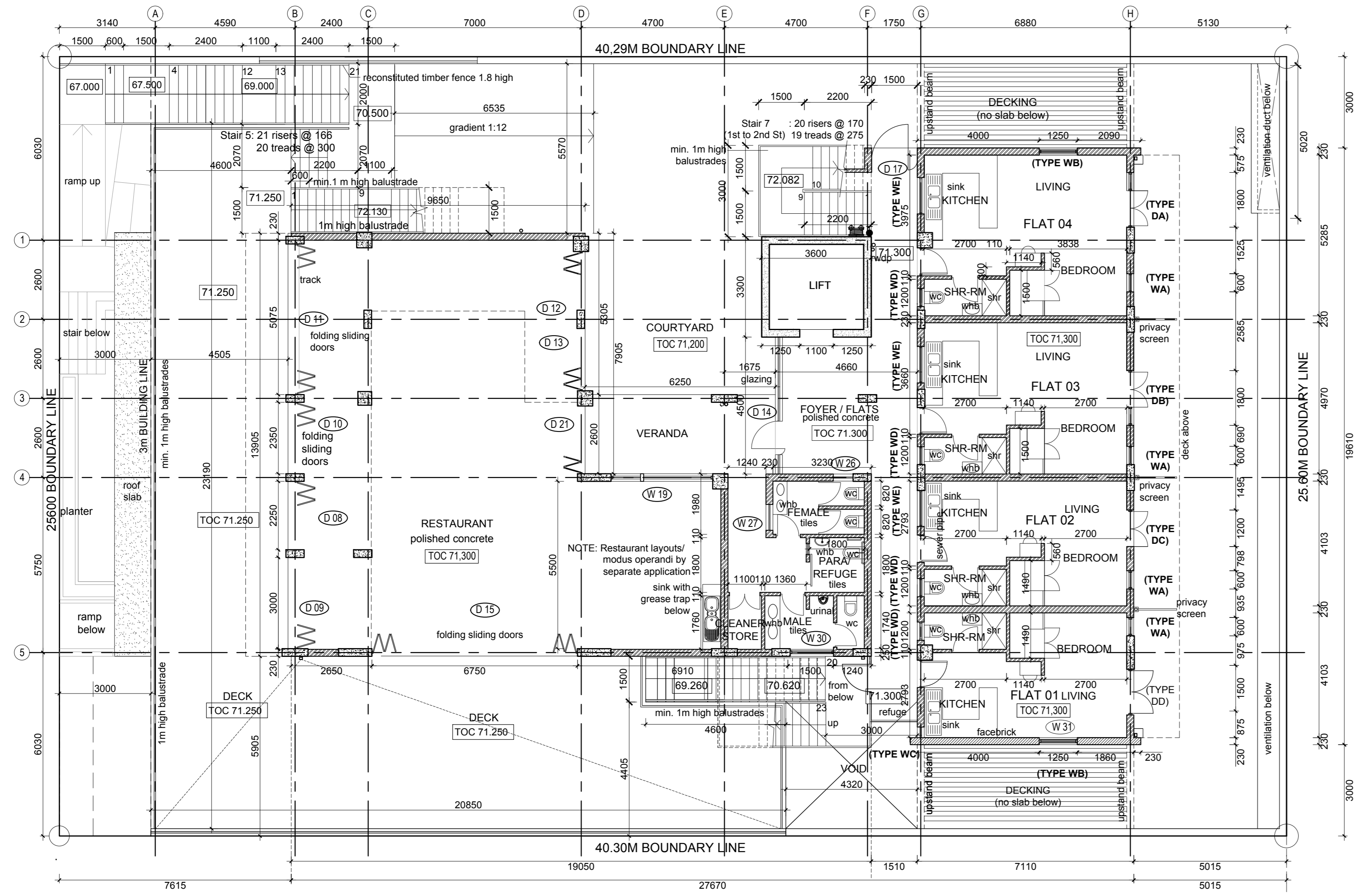
FIRST STOREY
