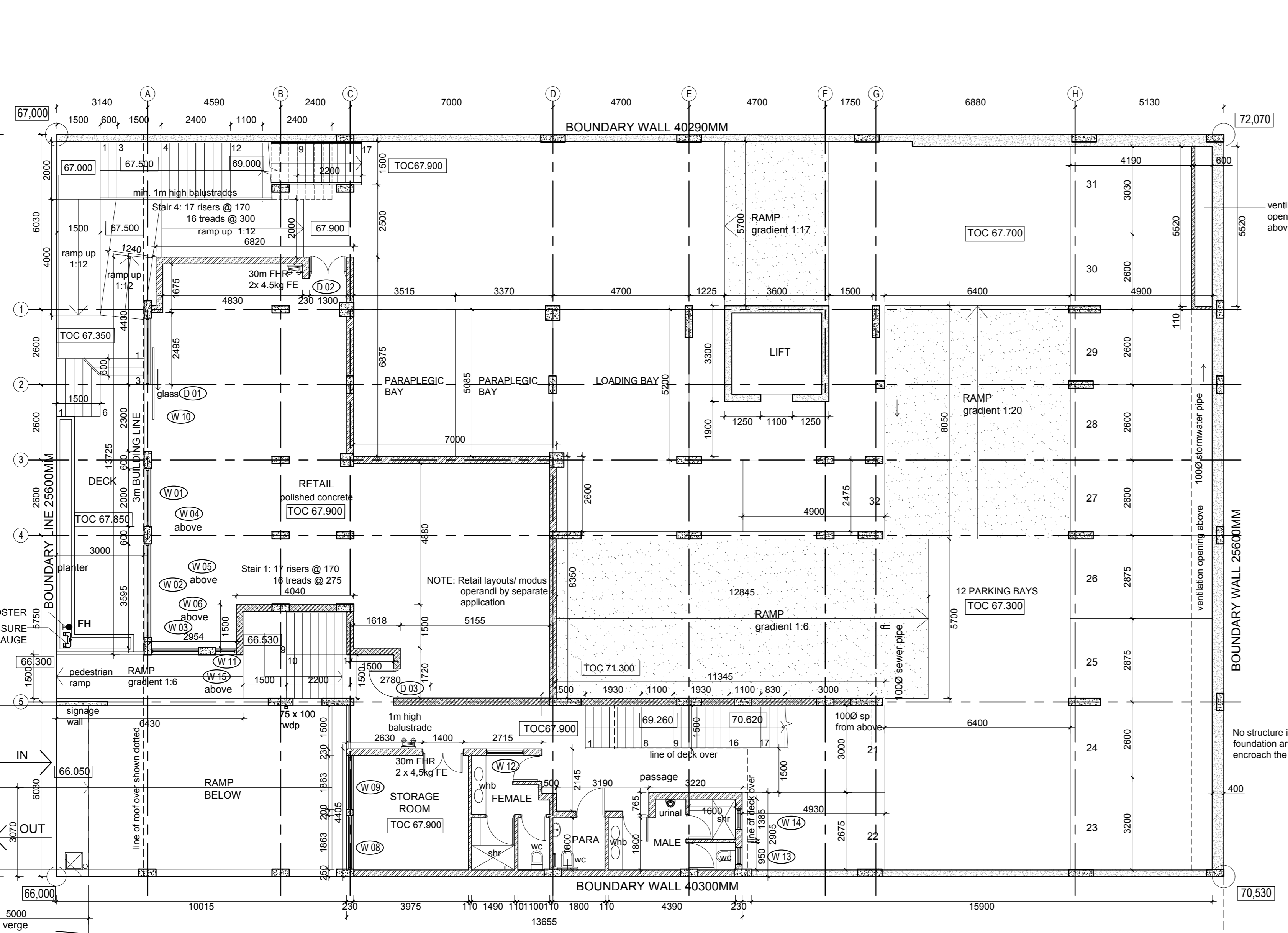
GROUND STOREY
